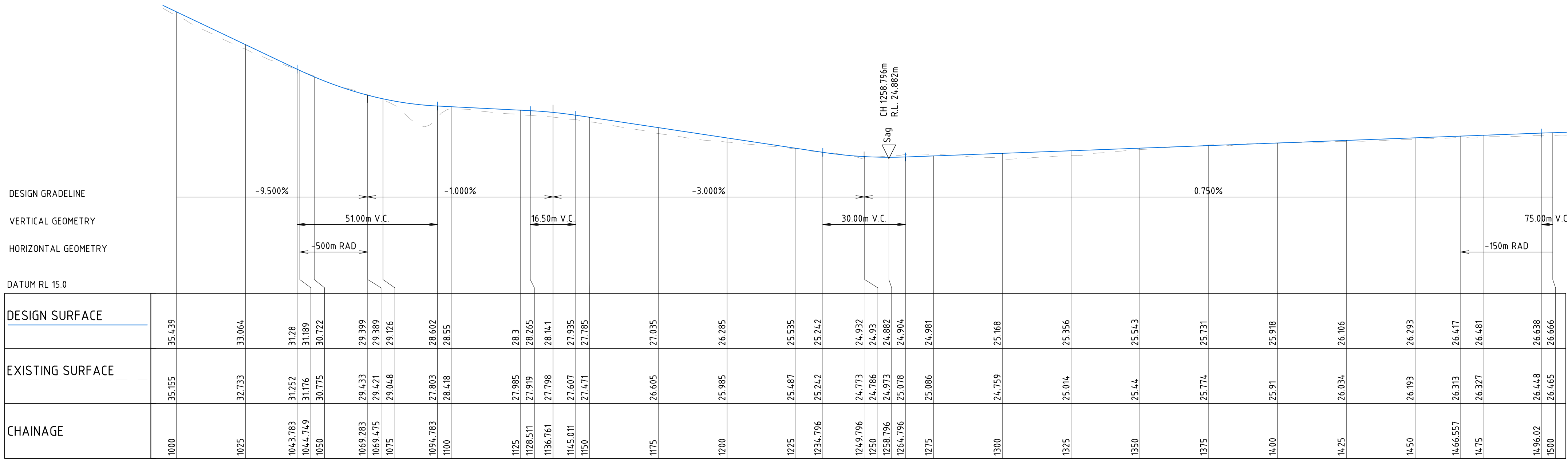
LONGITUDINAL SECTION ALONG MC11 HORIZONTAL SCALE 1:1000@A1 VERTICAL SCALE 1:200@A1
